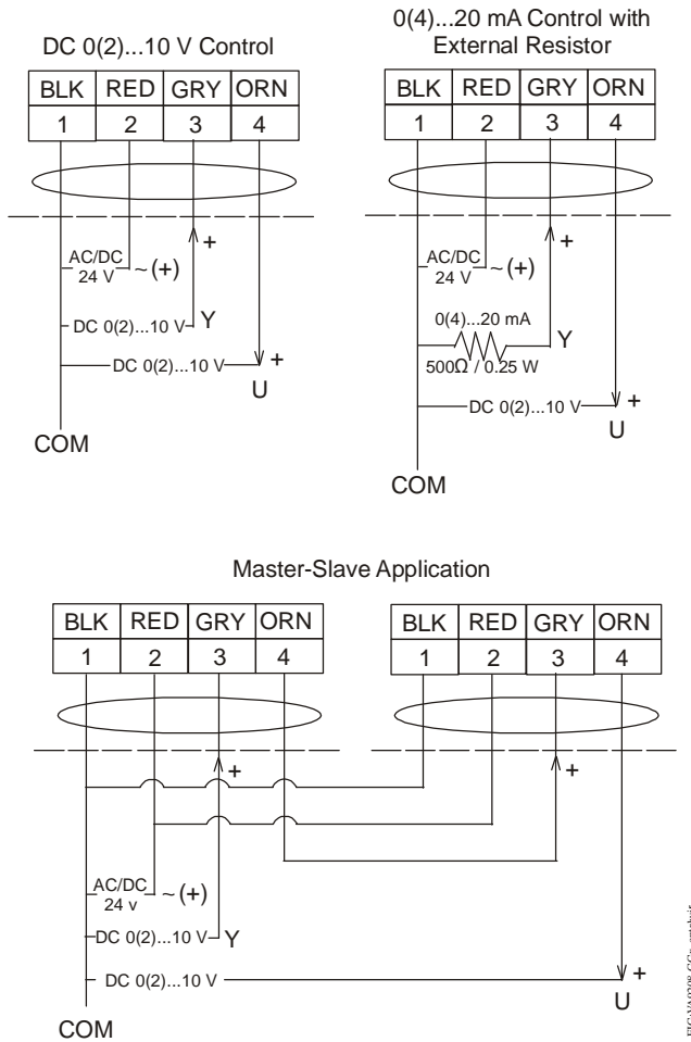
Figure 2: VA9203-GGx-2Z Control Wiring Diagrams
