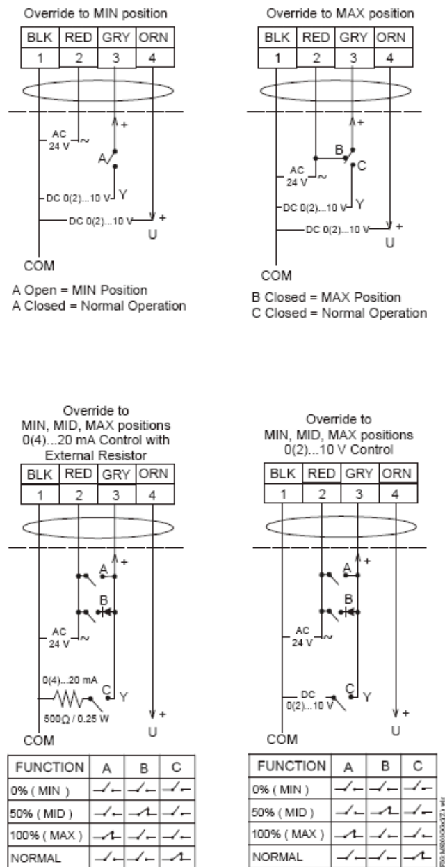
Figure 3: Control Wiring Diagrams (Overrides)
